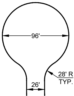
96' DIAMETER CUL-DE-SAC
