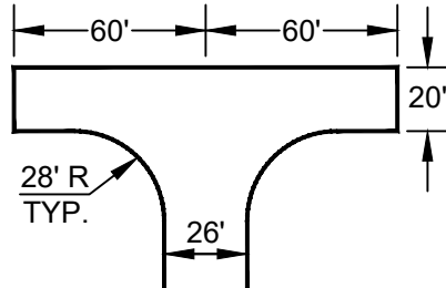
120' HAMMERHEAD
