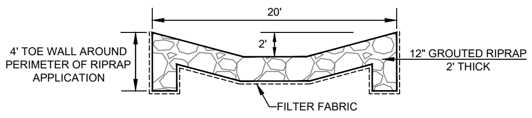
GROUDED RIPRAP
