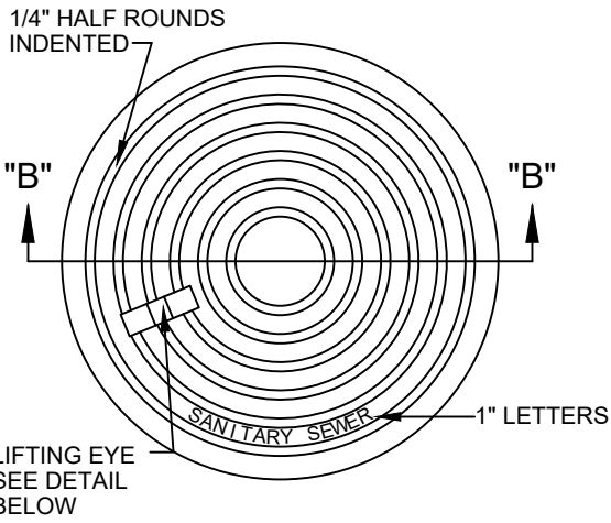
TOP OF COVER
