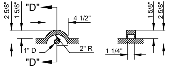
SECTION "C"- "C" SECTION "D"- "D" LIFTING EYE
