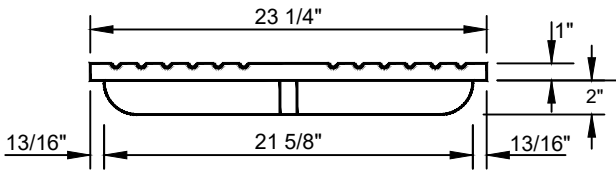
SECTION "B"- "B" MANHOLE COVER
